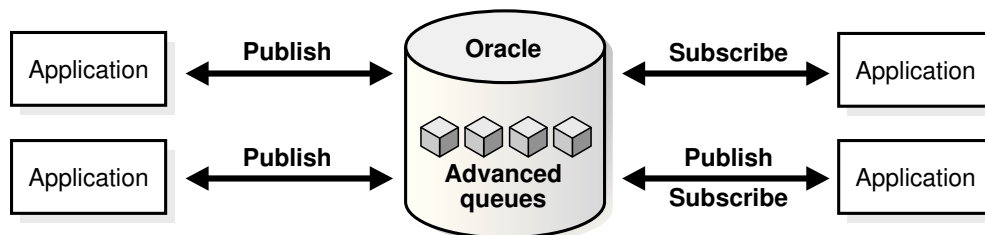
Figure 1-7 Publish/Subscribe Mode
