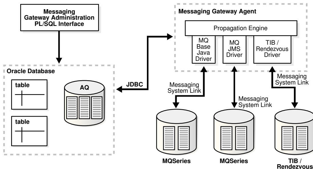
Figure 17-1 Messaging Gateway Architecture
