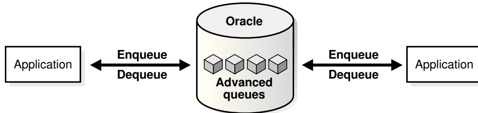
Figure 1-6 Point-to-Point Messaging
